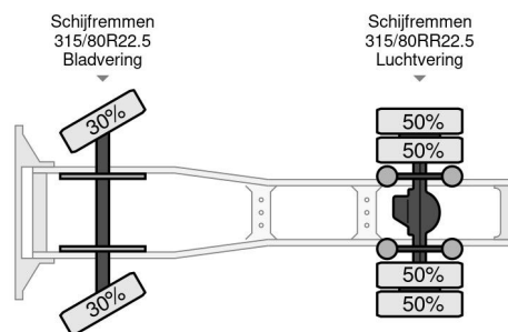
DAF XF 530 FT SPACE CAB ZF INTARDER
