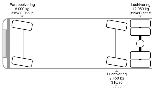
DAF CF 340 FAG MOL VDK Pu... 6x2
