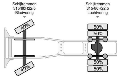
DAF XF 530 FT SPACE CAB ADR
