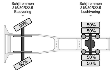
DAF CF 480 FT SPACE CAB
