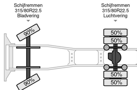
DAF CF 480 FT SPACE CAB
