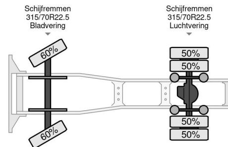
DAF XF 480 FT SUPER SPACE CAB
