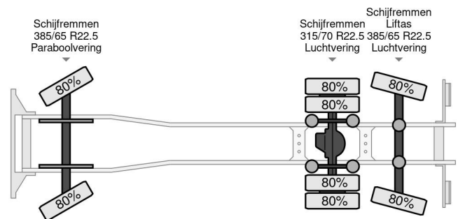
DAF XD 450 FAN 6x2 Road with AJK Loader JL20-5930A wi...
