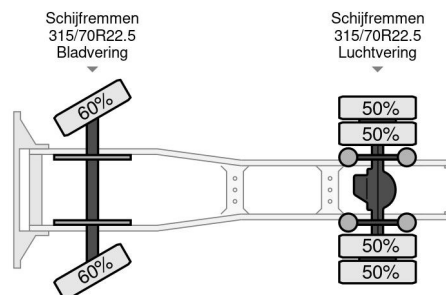
DAF XF 480 FT SUPER SPACE CAB, different location :... 4x2
