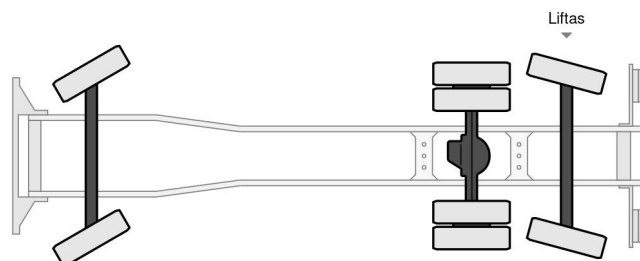
DAF XD 450 FAN FAssi F235A.2.23 E-Dynamic + TAM ... 6x2 Referenznummer: CHW-KR-11 - 2DWJ010
