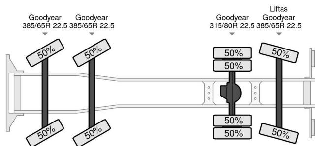
DAF CF 480 FAQ +Fassi Kraan F235A2.24 + Container... 8x2
